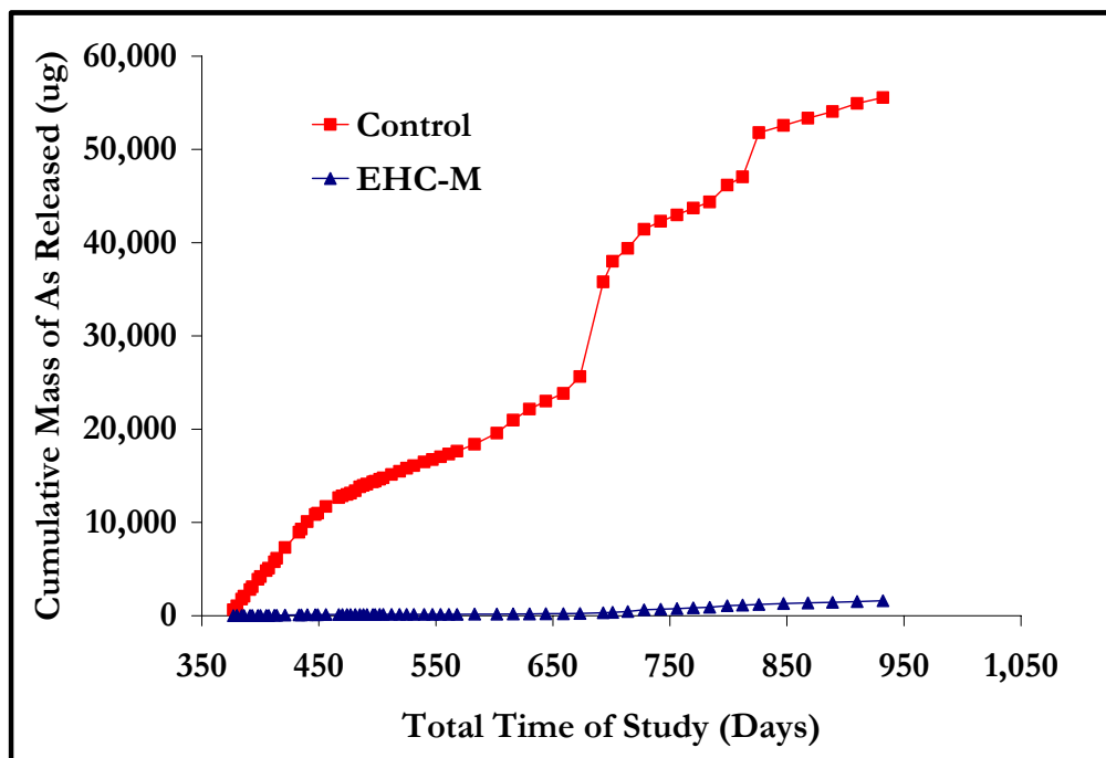
Figure 2. Cumulative mass of arsenic released from control and EHC-M columns in flow-through column study.
