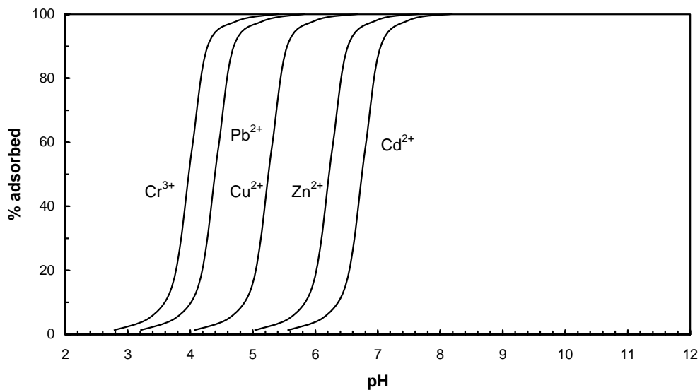
Figure 2. Adsorption of Cr 3+ , Cu 2+ , Cd 2+ , Zn 2+ , and Pb 2+ on hydrous ferric oxide as a function of pH. Each metal shows adsorption "edge"; at pH values below the edge, the ion is not adsorbed. At pH values above the edge, the ion is strongly adsorbed. High ratios of hydrous ferric oxide to adsorbing ion and an ionic strength of 0.1 M were assumed. (Data from Ref. 9).
