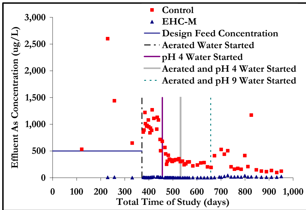
Figure 1. Influence of EHC-M and control on arsenic concentrations in groundwater in flow-through column study.
