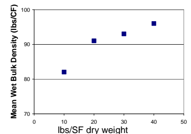
Figure 8. Typical Dry Bulk Density for AquaBlok HoleBlok+
